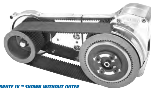
BRUTE IV™ SHOWN WITHOUT OUTER BELT GUARD (PP-419-P-AV), WHICH IS INCLUDED
